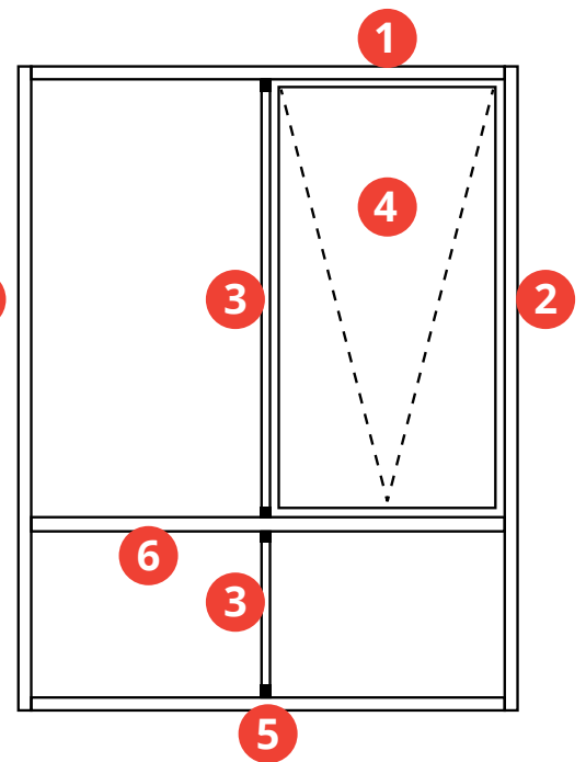
RESIDENTIAL AWNING WINDOW
